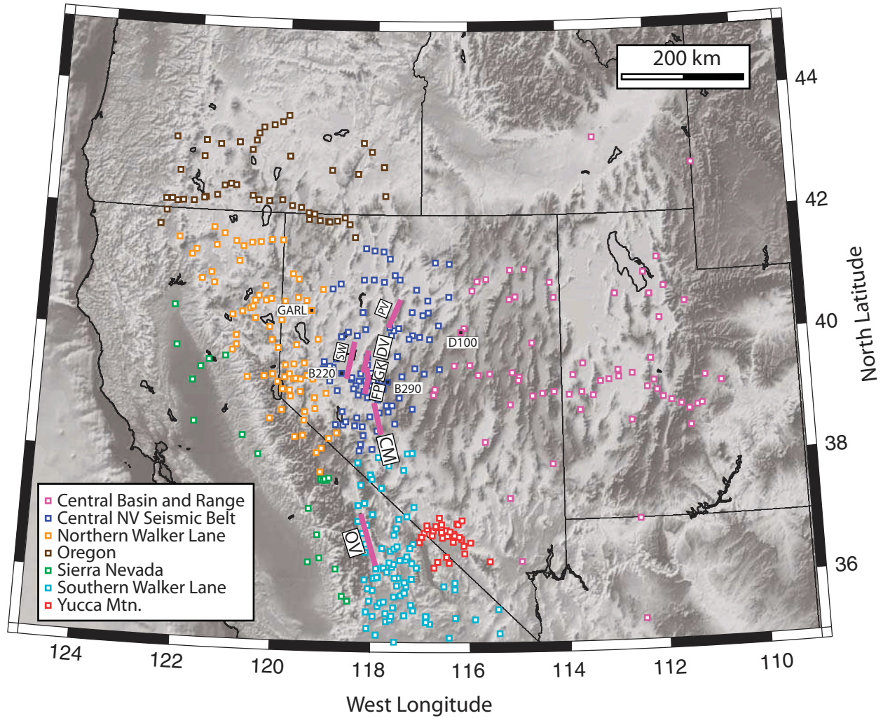
Figure 1. Horizontal velocities for global positioning system (GPS) sites used to constrain the viscosity of the Basin and Range lower crust and upper mantle. Site color designates the strain rate subnetwork discussed in text. Magenta line segments are the fault segments used to model the postseismic relaxation from the Central Nevada seismic belt historic earthquakes. See text for details of fault segments and coseismic slip parameters. Sites labeled GARRL, B220, B290, and D100 and having black interiors are discussed in the text. Fault segments are: CM—Cedar Mountain; DV—Dixie Valley; GK—Gold King–Louderback sequence; FP—Fairview Peak; OV—Owens Valley; PV—Pleasant Valley; SW—Stillwater sequence.
