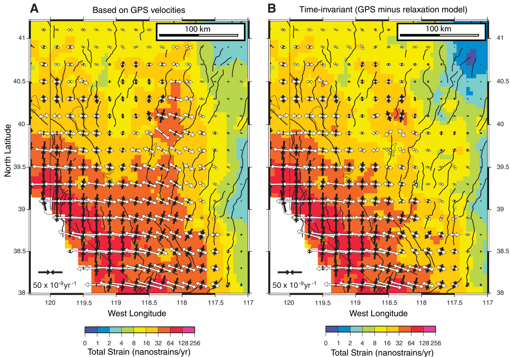
Figure 9. (A) Continuum strain rate model based on the global positioning system (GPS) velocity data. This is a detail of the map presented in Kreemer et al. (this volume). Other features are the same as B. (B) Same model except based on the time-invariant GPS velocity field obtained by subtracting the preferred relaxation model velocities ( \eta_{\text{LC}} = 10^{20.5} , \eta_{\text{UM}} = 10^{19} Pa·s) from the GPS velocities. The zone of deformation has become significantly more focused to the western edge of the Walker Lane belt.
