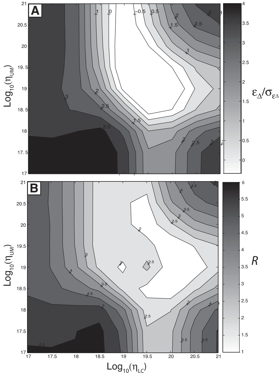
Figure 5. (A) Contour of the dilatational strain rate after correction for postseismic relaxation at the Central Nevada seismic belt normalized by its uncertainty as a function of lower-crustal ( \eta_{LC} ) and upper-mantle ( \eta_{UM} ) viscosity. Values greater than 2 indicate dilatation that is significantly larger than zero to 95% confidence. (B) Contour plot of R , the ratio of the scalar geodetic moment rate after correction for postseismic relaxation to the scalar geologic moment rate in the Central Nevada seismic belt.
