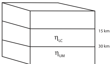
Figure 3. Rheological properties of our model as a function of depth. The uppermost layer (0–15 km) is assumed to be elastic; the lower crust (15–30 km) and upper mantle are assumed to be Maxwell viscoelastic. The elastic modulus \mu is obtained from the one-dimensional seismic model PREM (Dziewonski and Anderson, 1981), and viscosities of the lower crust \eta_{LC} and upper mantle \eta_{UM} are varied in a grid search.
