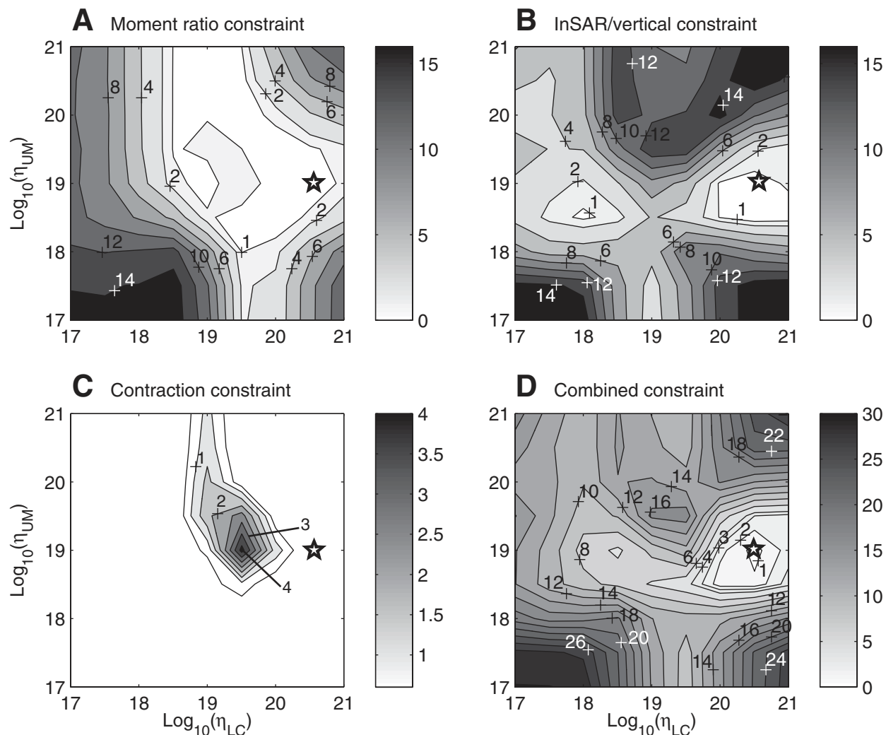
Figure 4. Model misfits as a function of lower-crustal ( \eta_{LC} ) and upper-mantle ( \eta_{UM} ) viscosity. (A) Contour of the first term of Equation 3, which depends on the ratio between geodetic and geologic scalar moment rate. Lower values indicate a better match between geologic and geodetic data. (B) Contour of the second term in Equation 3, which describes the misfit between the predicted vertical rate at the Central Nevada seismic belt and that measured by InSAR. (C) Contour of the third term in Equation 3, which is sensitive to the presence of undesirable time-invariant contractions in the areas surround the Central Nevada seismic belt. (D) The total constraint from all three data types combined using the method discussed in the text. Each panel has a star showing the preferred model ( \eta_{LC} = 10^{20.5} , \eta_{UM} = 10^{19} Pa-s).
