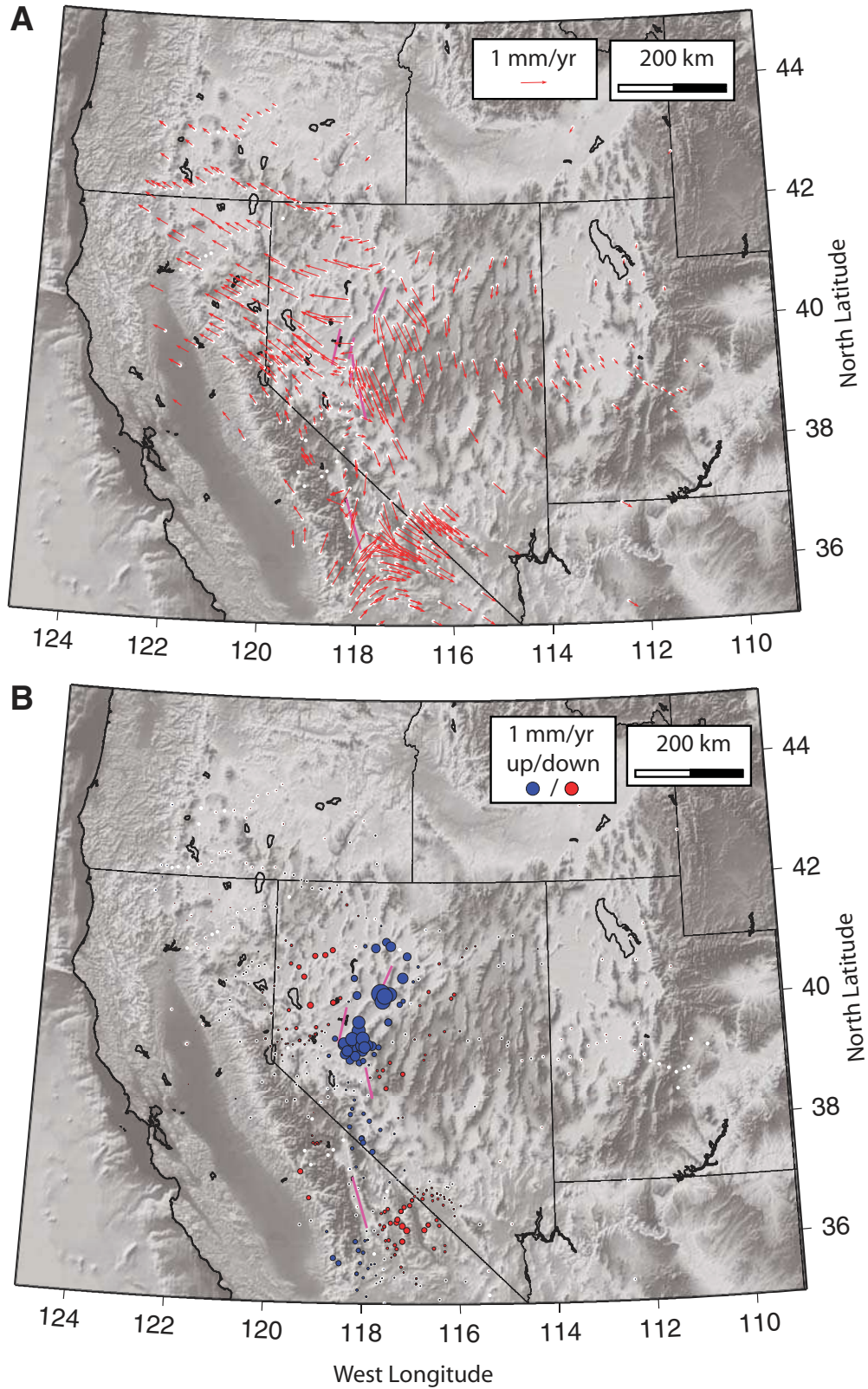
Figure 7. Postseismic relaxation velocities predicted from the preferred relaxation model ( \eta_{LC} = 10^{20.5} , \eta_{UM} = 10^{19} Pa-s), including the contributions from all the earthquakes considered in this study. (A) Red vectors show predicted horizontal velocity to the model faults (magenta line segments) at each global positioning system (GPS) site in the compilation of Kreemer et al. (this volume). (B) Vertical motion is shown blue for uplift, red for subsidence. Size of the circle indicates the vertical rate.
