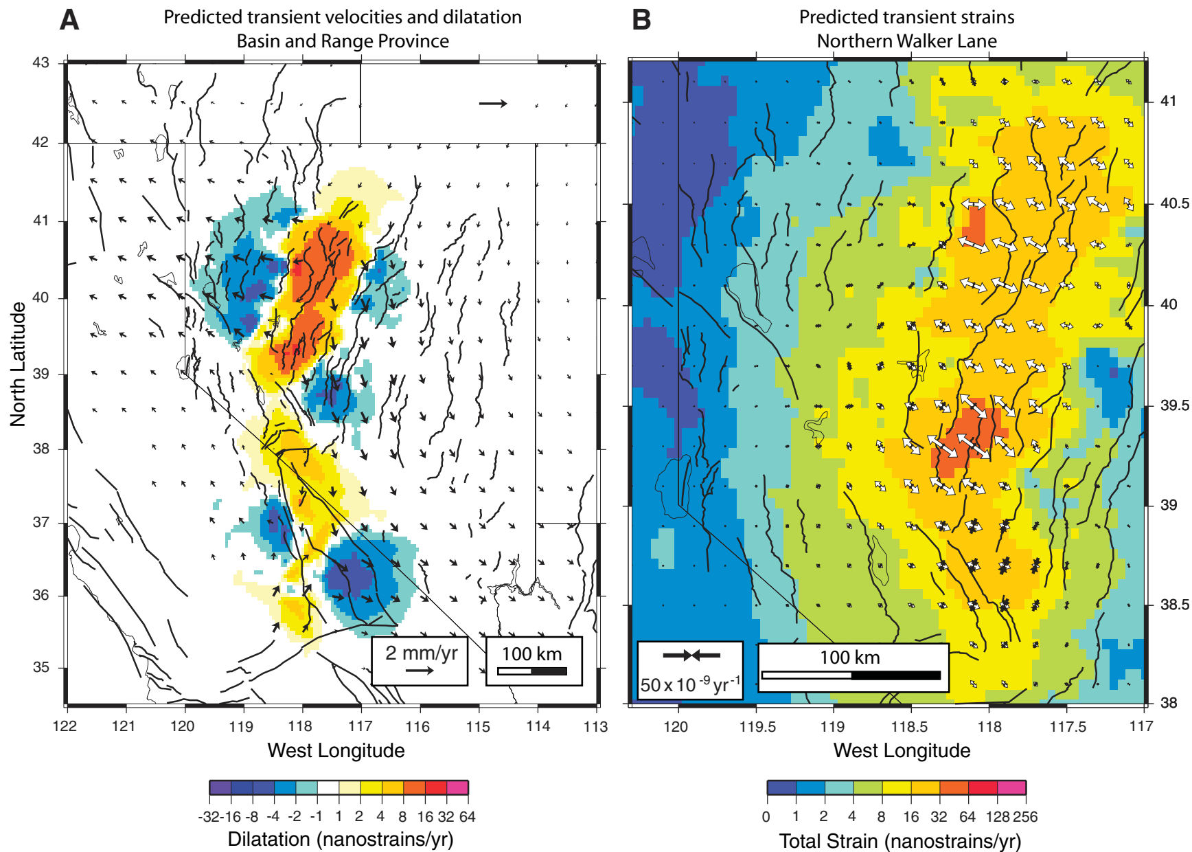
Figure 8. (A) Dilatational strain rates predicted from the preferred relaxation model velocities ( \eta_{LC} = 10^{20.5} , \eta_{UM} = 10^{19} Pa·s). This map was created using the same global positioning system (GPS) site locations as the model of Kreemer et al. (this volume), so that the effects of station distribution on the strain modeling are included. Black arrows indicate the relaxation velocities interpolated onto a regular grid. Quaternary faults are shown with black line traces. State borders and major lakes are shown with faint lines. (B) A detailed view of the northern Walker Lane. The colors now represent the amount of total strain rate, which contains both horizontal shear and dilatation. Black arrow pairs indicate tensor contraction; white arrows indicate tensor extension.
