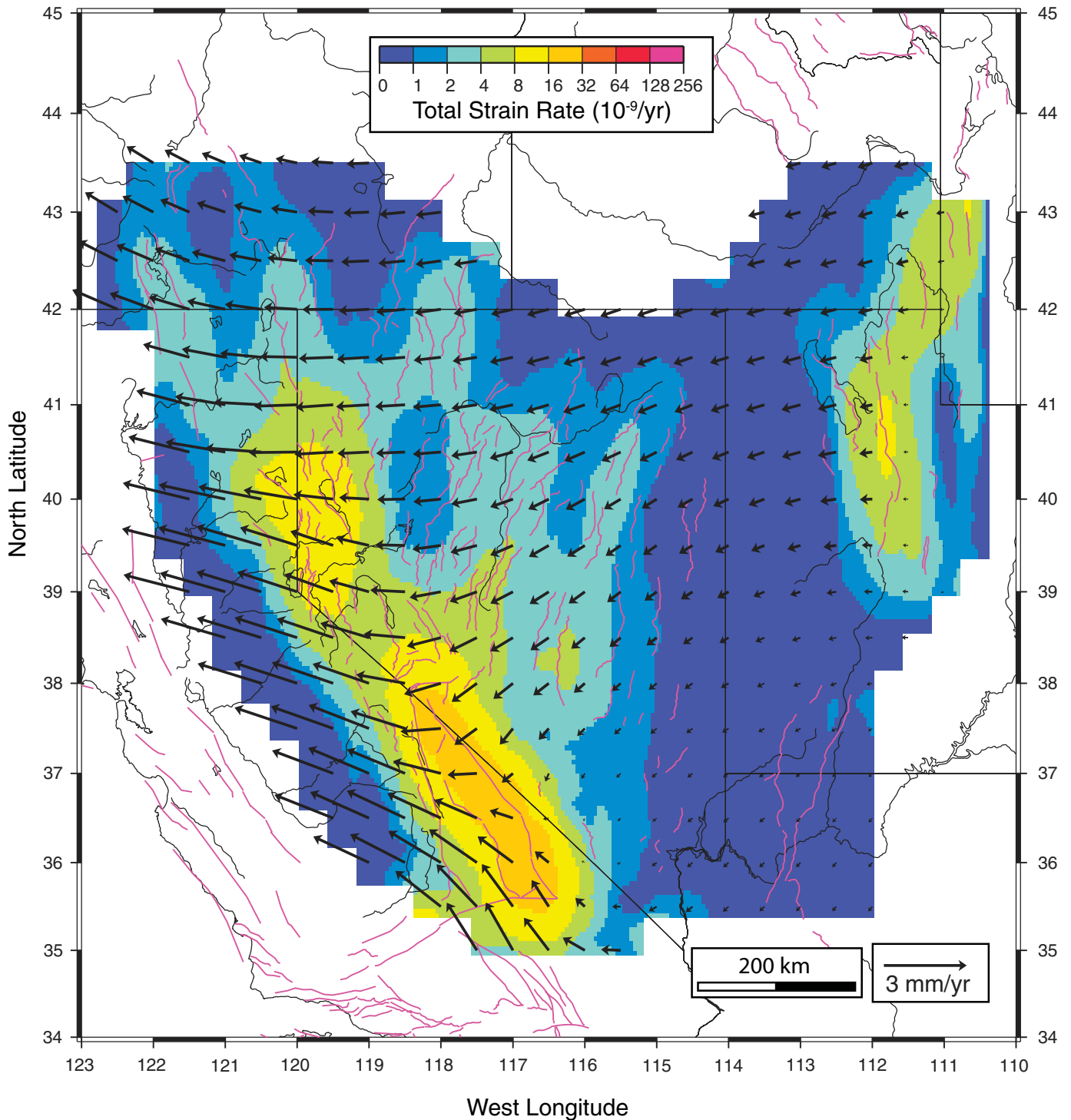
Figure 2. Strain rate field inferred from the paleoseismic databases of the U.S. Geological Survey and dePolo and Anderson (2000). Black arrows are velocities with respect to North America on a regular grid that result from integration of the strain rates. Colors are the second invariant of the strain rate (includes shear and dilatation). Magenta line traces are faults in the database. Note that the finger of higher strain rates near longitude 117°W and latitude 39°N lies east of the Central Nevada seismic belt.
