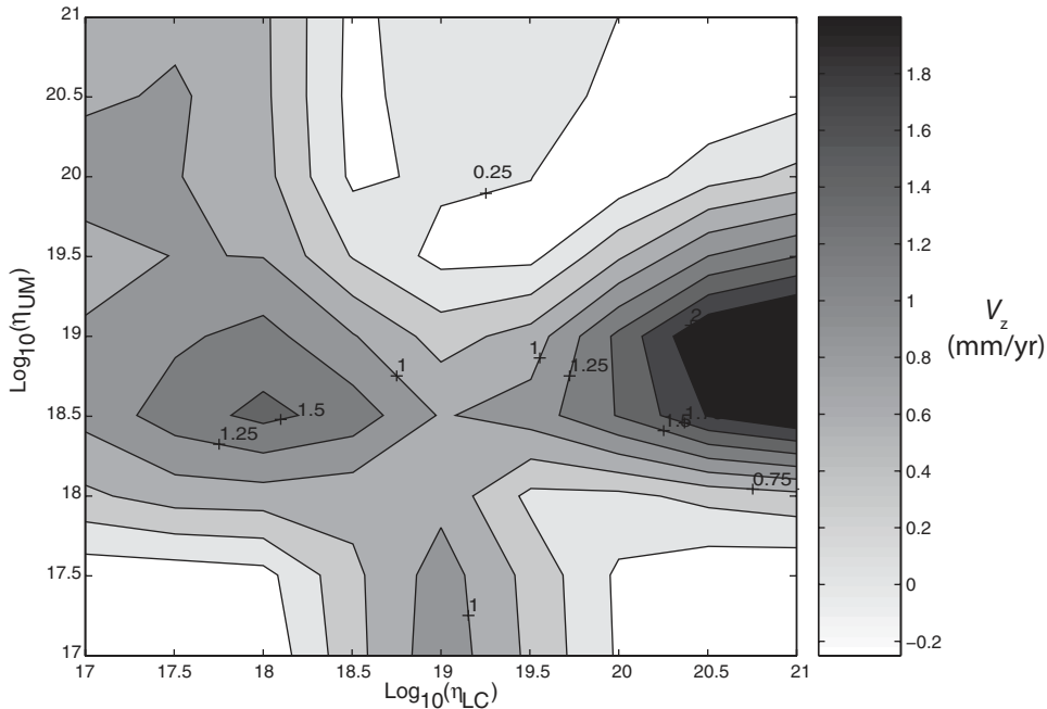
Figure 6. Contour of uplift rate ( V_z ) at the Central Nevada seismic belt predicted from the relaxation model as a function of lower-crustal ( \eta_{LC} ) and upper-mantle ( \eta_{UM} ) viscosity.
