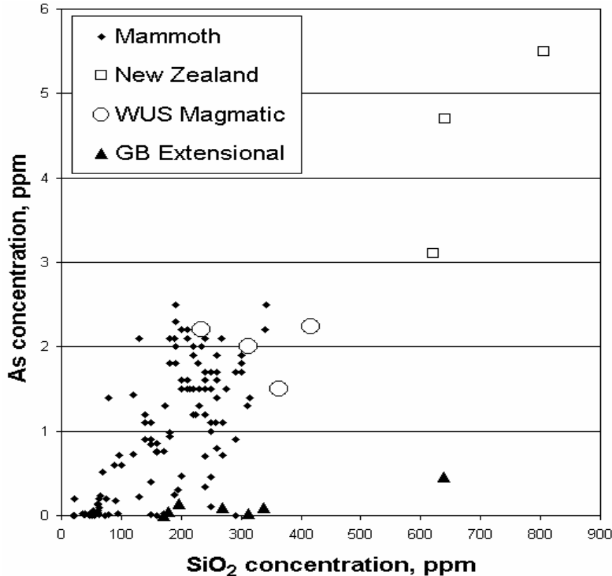
Figure 1: Plot of As content of geothermal fluids vs. ppm SiO 2 (as a proxy for maximum temperature) for a variety of geothermal systems. GB = Great Basin; WUS = Western US. The WUS Magmatic group includes data from Steamboat NV; Roosevelt, UT; Yellowstone, WY; and Shasta, CA. All systems except those included as GB extensional are considered to be magmatic.
