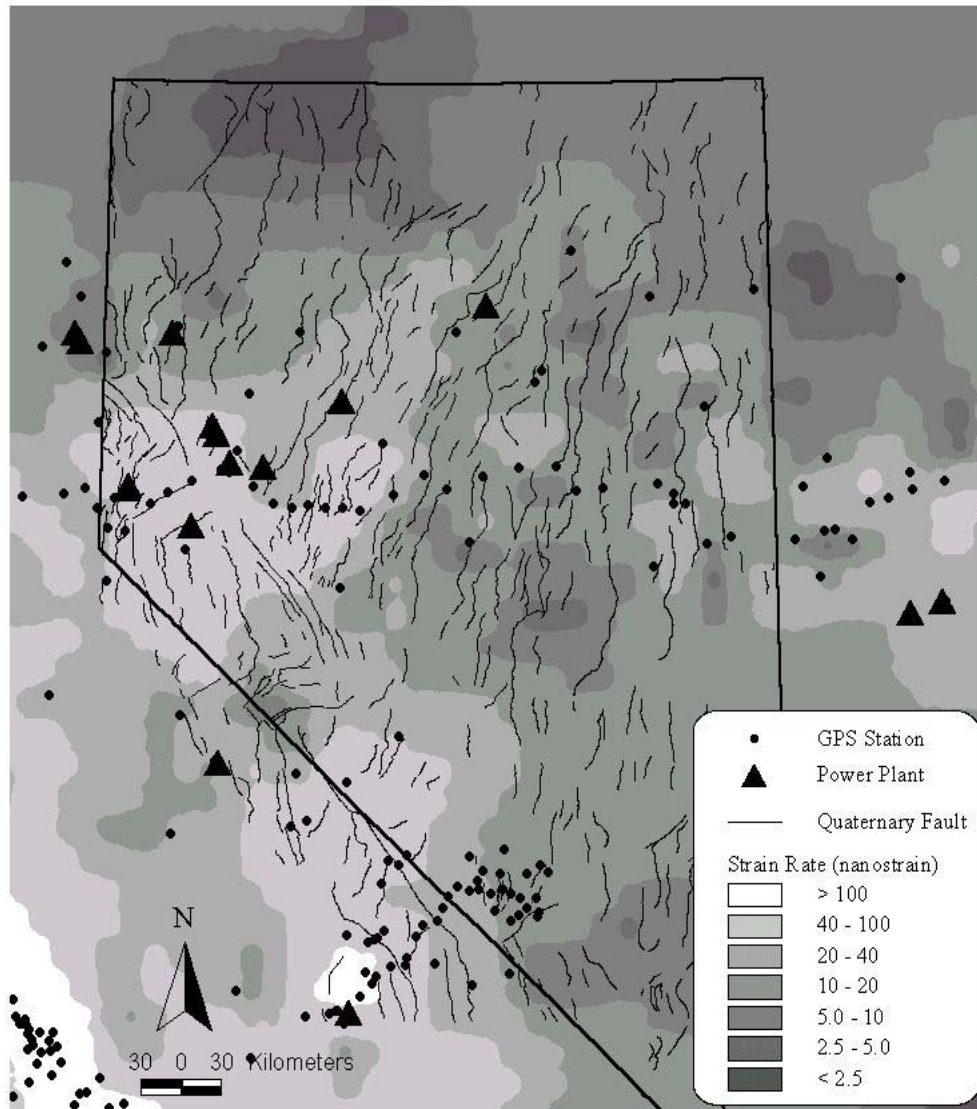
Figure 1. Map of the magnitude of strain rates in the Great Basin study area (Nevada border shown for reference) based on site velocity data from GPS stations shown. Higher strain rates are indicated by lighter shades. Superimposed are geothermal power-producing sites. Quaternary faults have been digitized and are superimposed to illustrate the potential for defining a continuous field of favorable orientations with respect to the strain tensor field. Note that strain rate can only be interpreted with resolution at the same spatial scale as the distance between neighboring GPS stations, which varies considerably with location.
