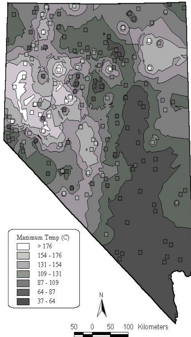
Figure 2. Trend surface of maximum geothermal temperatures. Locations of geothermal systems used for contouring are shown with squares. Method of surface interpolation was inverse distance weighting, with power of 1, using nearest 5 neighbors.
